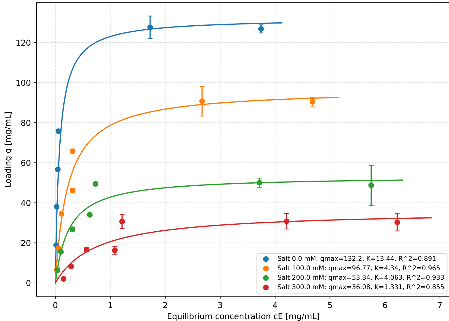
Loading Isotherms - Experiment 5016 at 280 nm
